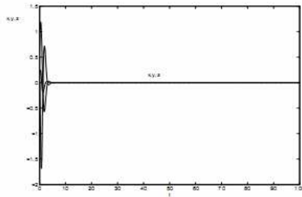
Figure 1: The time response of the states x, y, z of the controlled system (2.2), where \bar{x}=0, \bar{y}=0, \bar{z}=0 .
